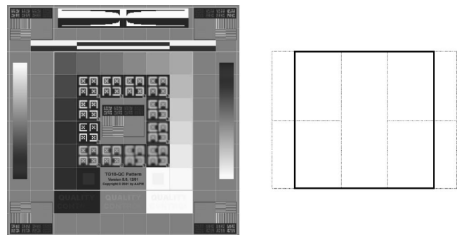
FIG. 2. Spatial measurements for the quantitative evaluation of geometric distortions using the TG18-QC test pattern. The small squares with dashed lines (- -) define the four quadrants of the pattern, and the large square at the center encompassing the luminance patches is the one to be used for geometric distortion characterization within the whole image.
