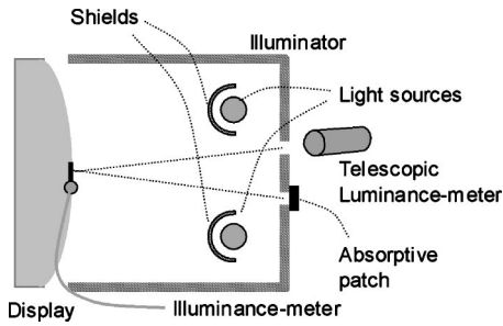
FIG. 4. Typical illuminating device used for the measurement of the diffuse reflection coefficient of a display device.
